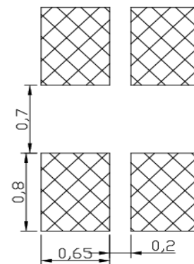
Figure 1. IN-S66TBTRGB Solder Pattern
