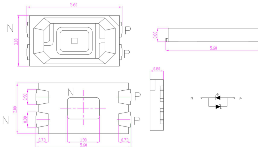
Figure 2. INV-P53CTRHIR Package Dimensions
