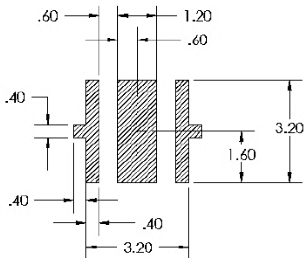
Recommended Stencil Pattern(Hatched Area is Opening)
