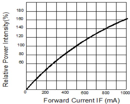
Relative Radiant Flux vs. Forward Current ( T_a=25^\circ\text{C} )
