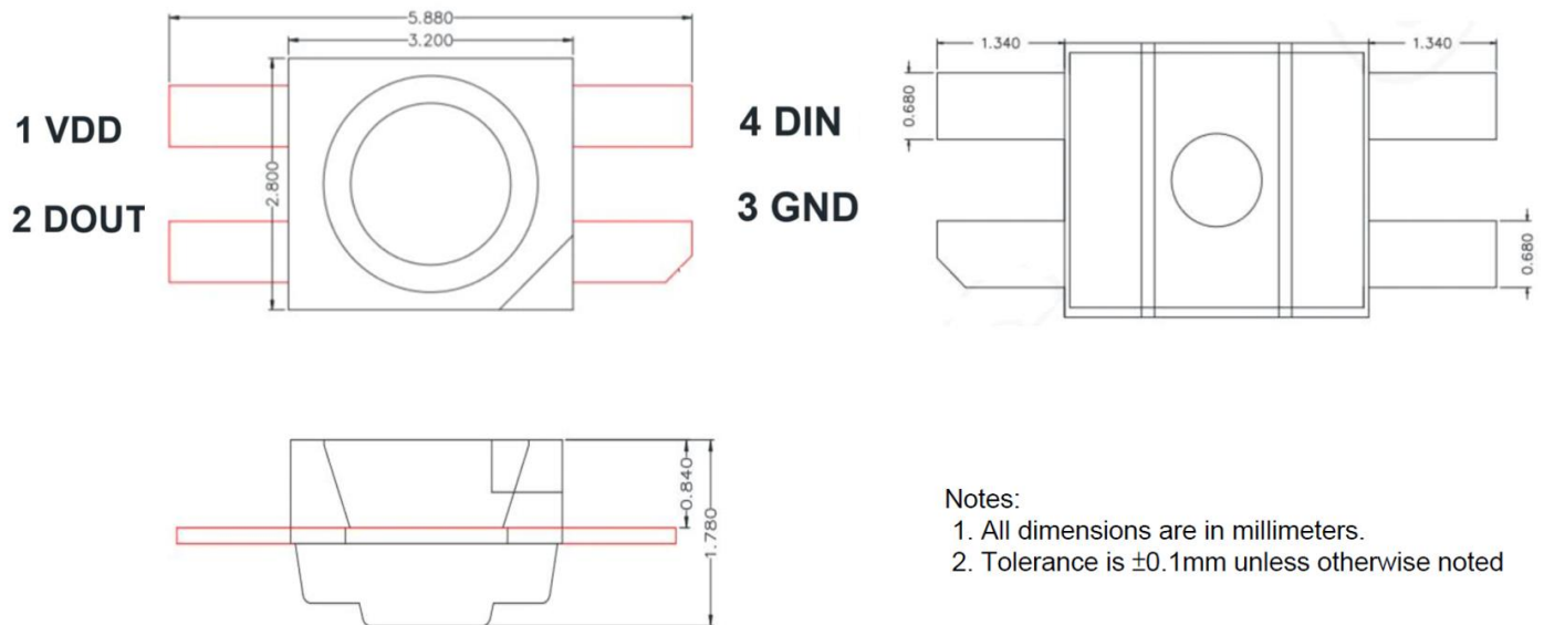
Figure 1. IN-PI32TAR(X)R(X)G(X)B Package Outline Dimensions
