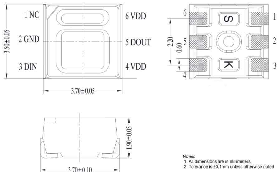
Figure 1. IN-PI33QBTPRPGBPBW-XX Package Outline Dimensions
