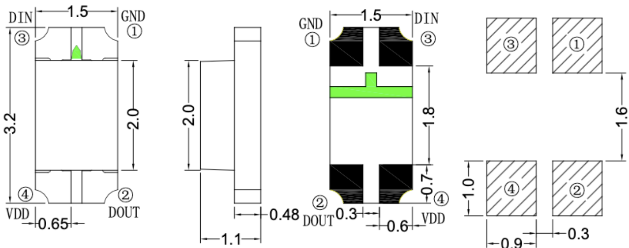
Figure 1. IN-PIS126ATPB Package Outline Dimensions
