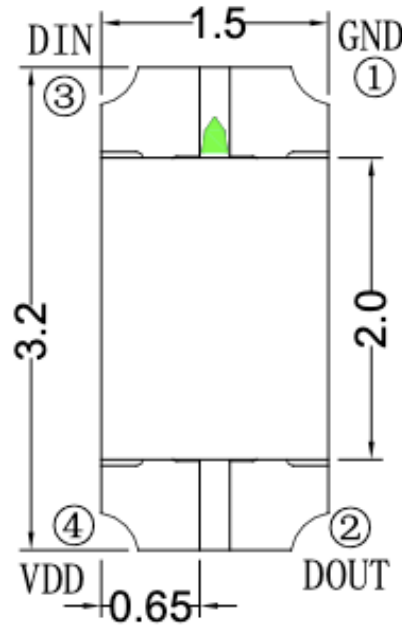
Figure 2. IN-PIS126ATPB Pin Configuration
