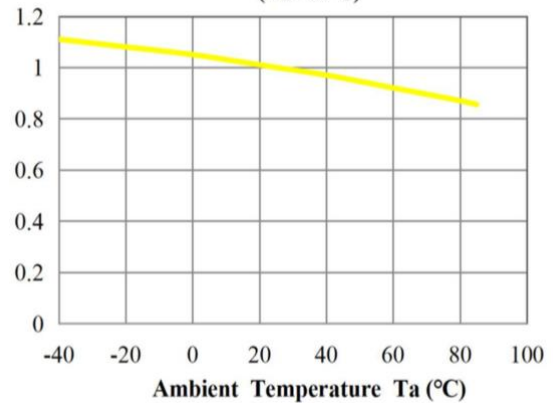
Relative Intensity VS. Ambient Temperature (Ta=25°C)
