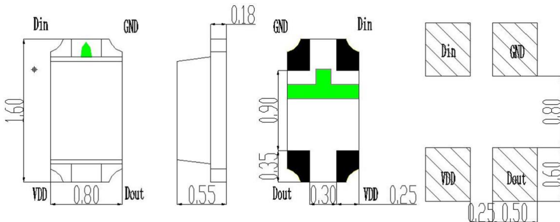
Figure 1. IN-PIS63BTPY Package Outline Dimensions
