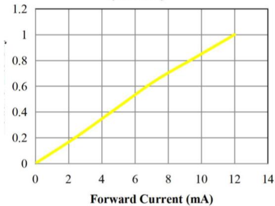
Relative Intensity VS. Forward Current (Ta=25°C)
