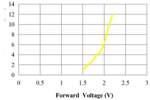
Forward Current VS. Forward Voltage (Ta=25°C)
