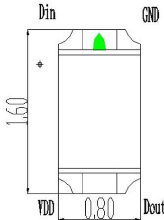
Figure 2. IN-PIS63BTPY Pin Configuration
